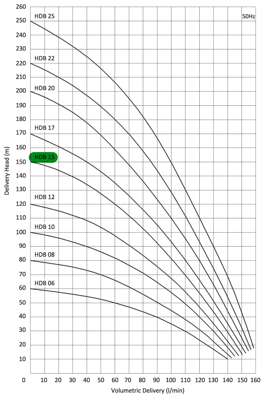
Performance Curve
